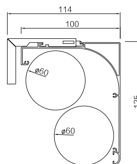
White or Fabric wrapped Z3 ( day&night )
