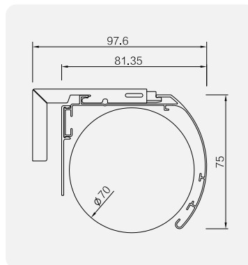
White S2/Fabric wrapped S3
