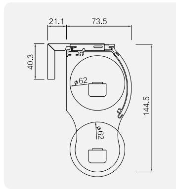
Fabric inserted Z1 ( day&night )
