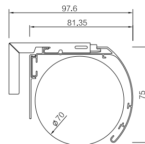
White S2/Fabric wrapped S3
