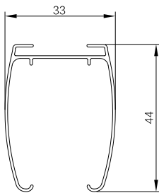
Cordless Headrail No Drill Blinds
