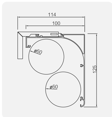
White or Fabric wrapped Z3 ( day&night )
