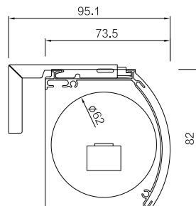
Fabric inserted S1
