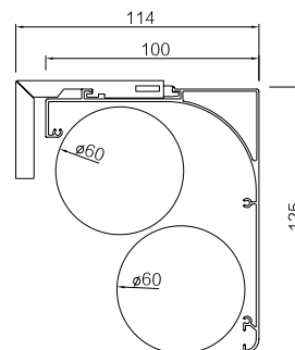
White or Fabric wrapped Z3 ( day&night )
