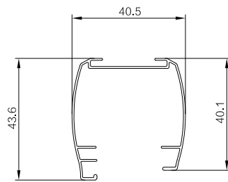
Bead Chain/ Motorized Headrail No Drill Blinds
